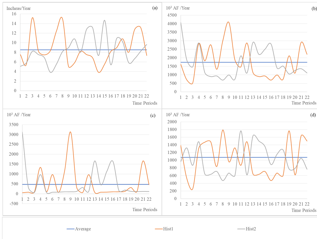
Figure 20. Simulated annual surface water availability and rainfall in the region. (a) regional rainfall; (b) Kings River flow; (c) San Joaquin River flow; (d) Friant-Kern Canal flow.
